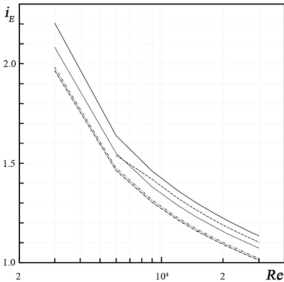
Fig.3. The variation of i_E with Reynolds number. Experimental results of Garcia et al. [6].
