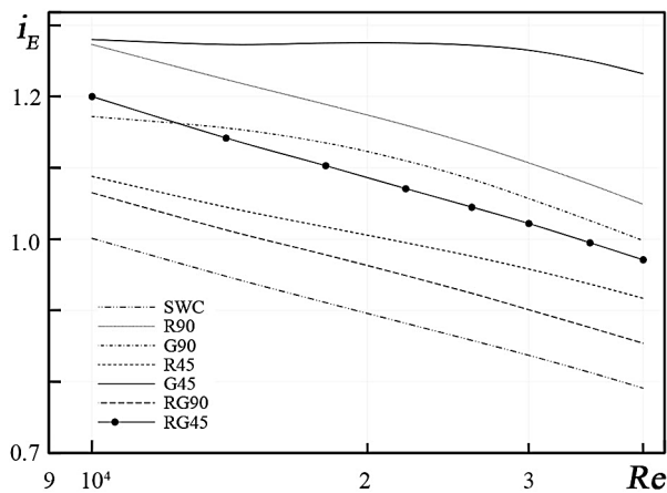
Fig.8. The variation of i_E with Reynolds number. Experimental results of Chang et al. [12], p/D_i = 1.0 .
