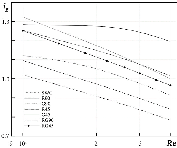
Fig.7. The variation of i_E with Reynolds number. Experimental results of Chang et al. [12], p/D_i = 0.5 .
