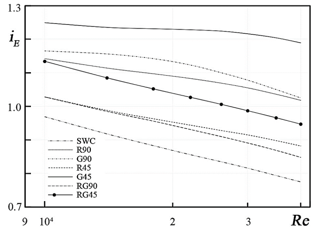
Fig.9. The variation of i_E with Reynolds number. Experimental results of Chang et al. [12], p/D_i = 1.5 .
