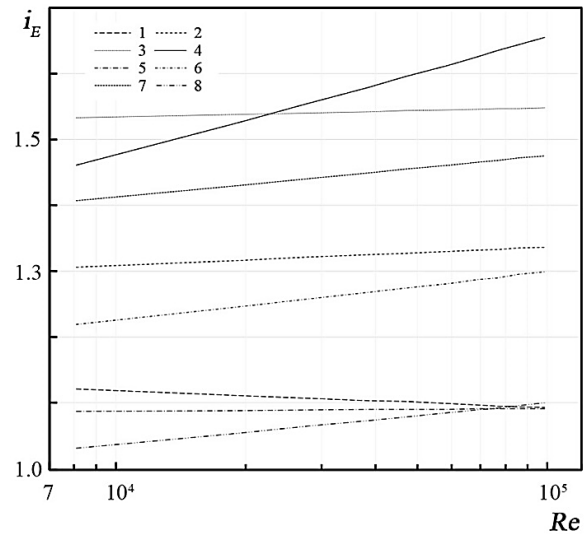
Fig. 1. The variation of i_E with Reynolds number. Experimental results of Sethumadhavan and Rao [3]
