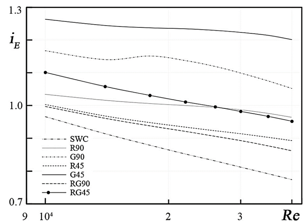
Fig.10. The variation of i_E with Reynolds number. Experimental results of Chang et al. [12], p/D_i = 2.0 .
