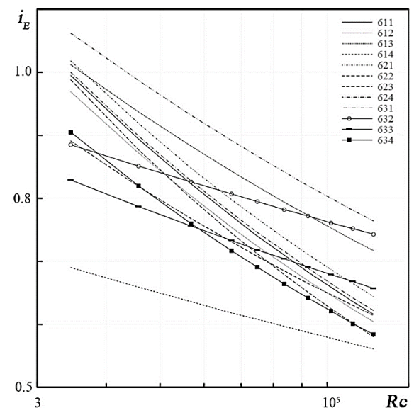
Fig.2. The variation of i_E with Reynolds number. Experimental results of Prasad and Shen [4].
