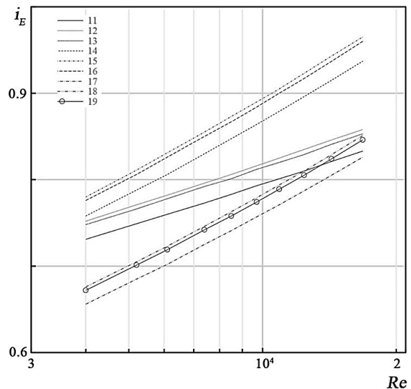
Fig.6. The variation of i_E with Reynolds number. Experimental results of San Jung-Yang et al. [11], Pr = 0.7 .
