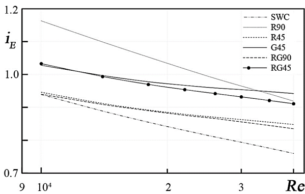
Fig.11. The variation of i_E with Reynolds number. Experimental results of Chang et al. [12], p/D_i = 2.5 .
