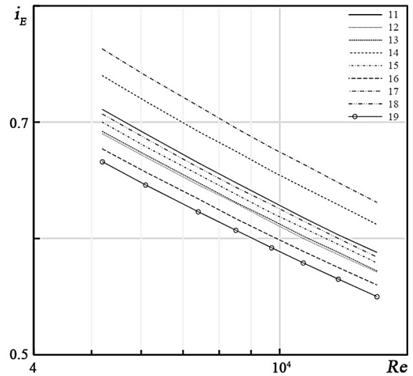
Fig.5. The variation of i_E with Reynolds number. Experimental results of San Jung-Yang et al. [11], Pr = 6.2 .
