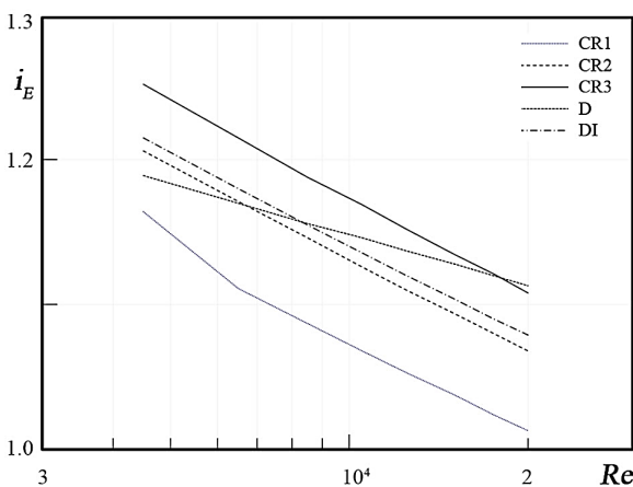
Fig.4. The variation of i_E with Reynolds number. Experimental results of Eiamsa-ard S. et al. [10].
