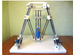
b) - frame layout five coordinate drill-mills machine-tool with MPS [5, 7]
