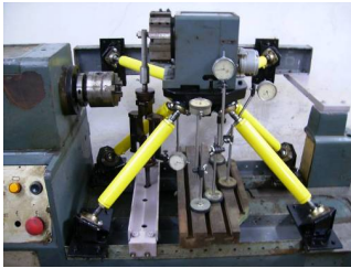
c) - multi-purpose machine-tool hexaglide [2, 7, 11]
