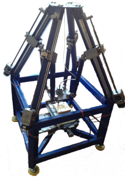
b) - frame layout five coordinate drill-mills machine-tool with MPS [5, 7]
